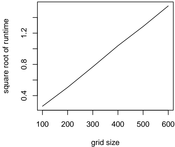
runtimes of dynamic function (sqrt)
