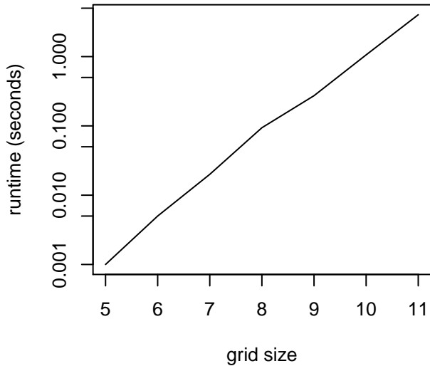
runtimes of recursive function (log)
