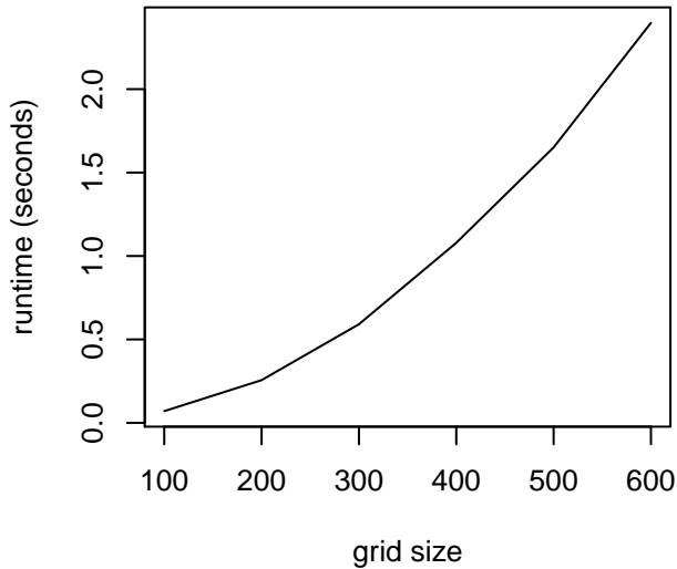
runtimes of dynamic function
